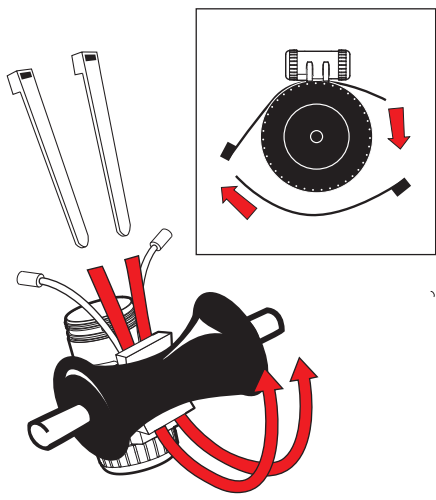
8. Attach to hub, for large hub use 4 straps.
